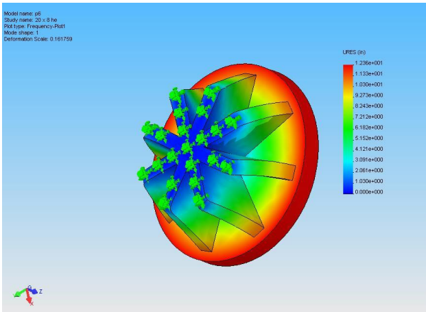
3D Modal Plot for Resonance Testing
